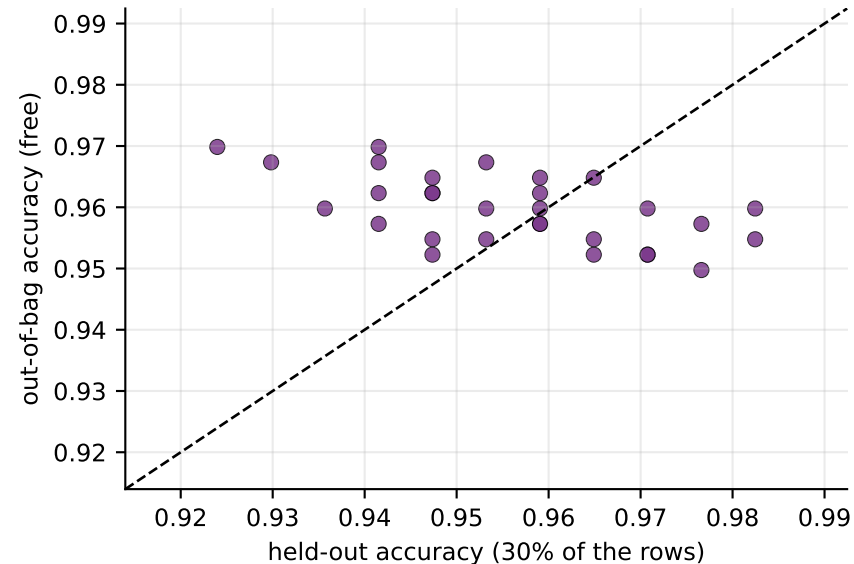
30 random splits of breast_cancer
