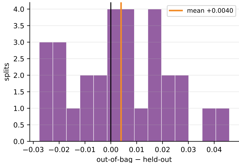
The free estimate is close and not systematically high
