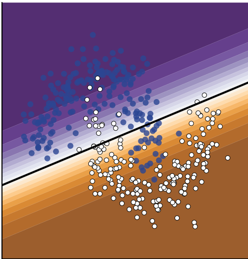
MLP 32-32, identity 1058 parameters accuracy 0.8775
