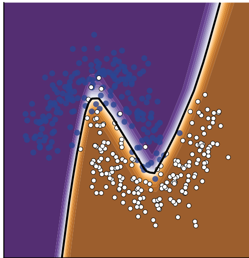
MLP 32-32, ReLU 1058 parameters accuracy 0.9625
