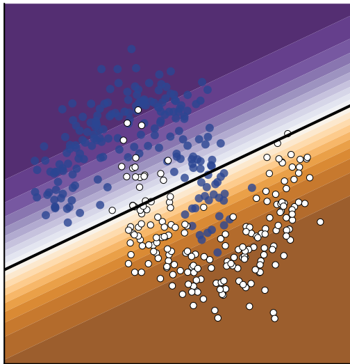
logistic regression 3 parameters accuracy 0.8750
