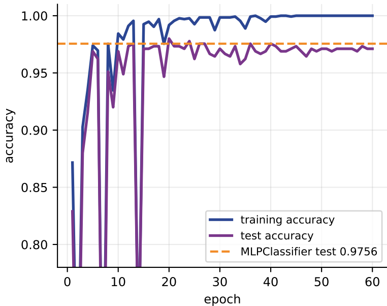
64-32-10 on load_digits, 2410 parameters
