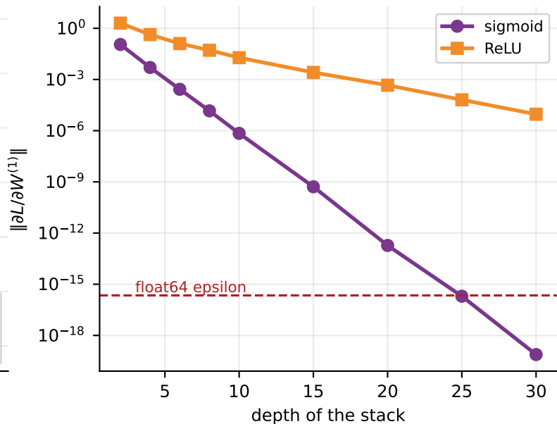
first-layer gradient against depth
