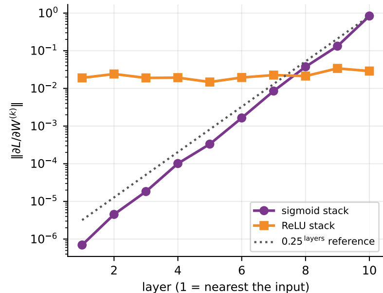
ten layers, identical weights, only the activation differs
