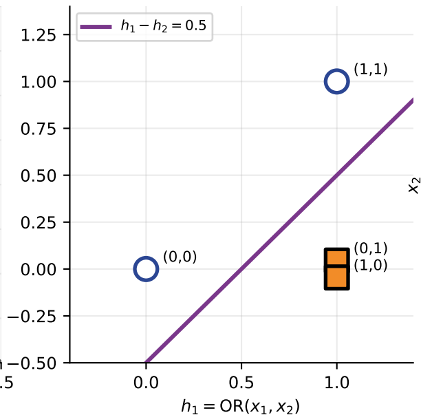
after one hidden layer: (0,1) and (1,0) coincide
