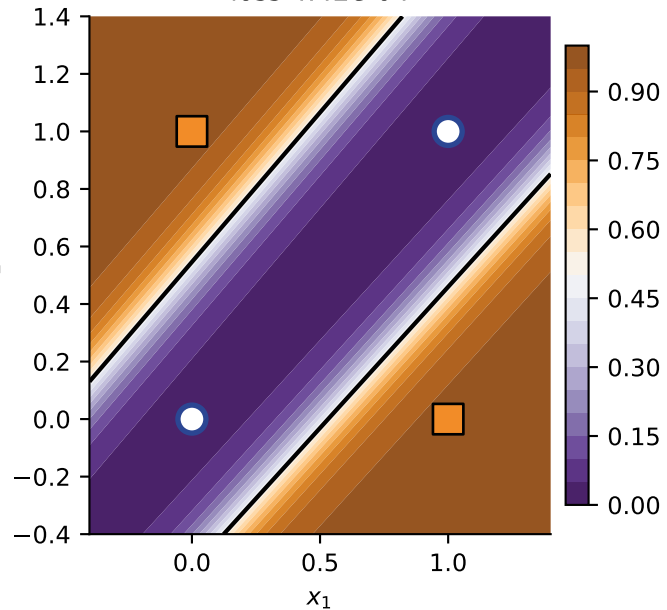
2-2-1 sigmoid network, trained: loss 4.42e-04
