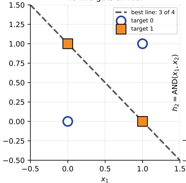
XOR in the input plane: no line gets all four
