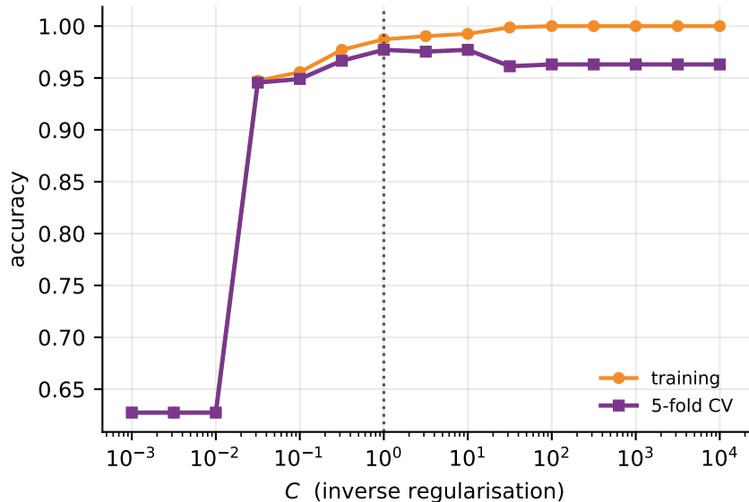
RBF SVM on breast cancer, scaled
