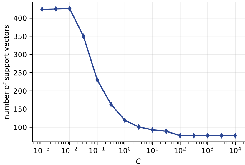
Large C keeps fewer points
