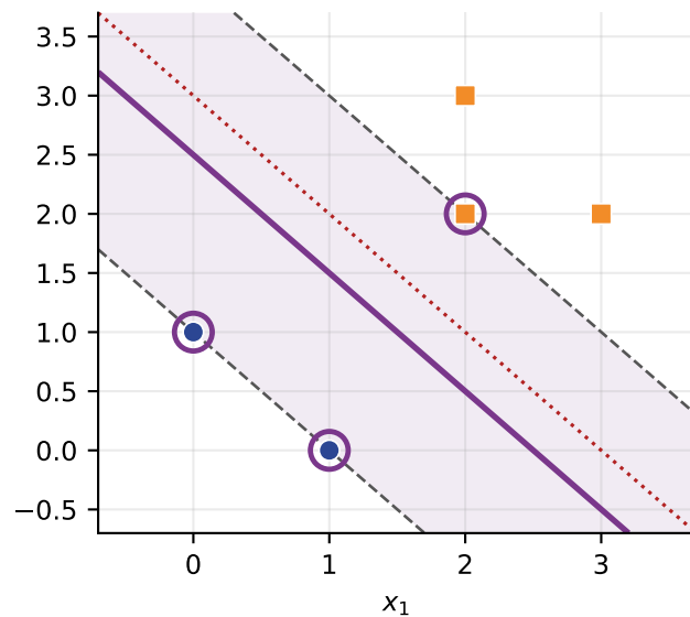
without A (1, 1) -- a SV
