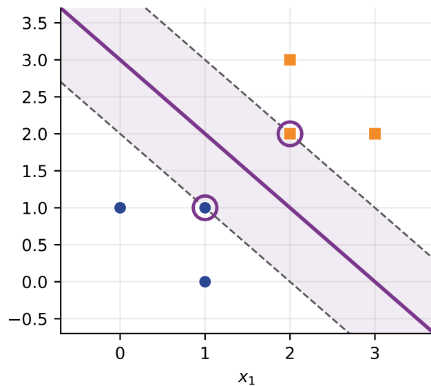
all six points
