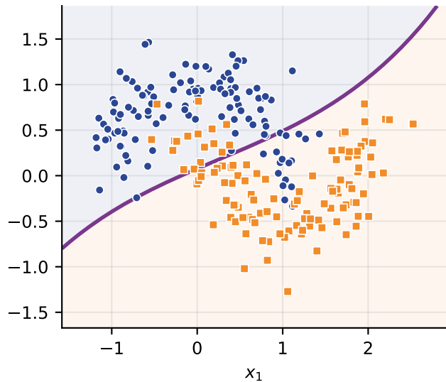
\gamma = 0.1 : train 0.8542, CV 0.8542 103 SVs
