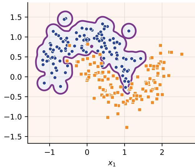
\gamma = 100 : train 0.9917, CV 0.9125 212 SVs
