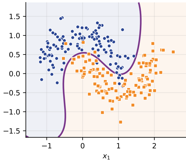
\gamma = 1 : train 0.9583, CV 0.9458 64 SVs
