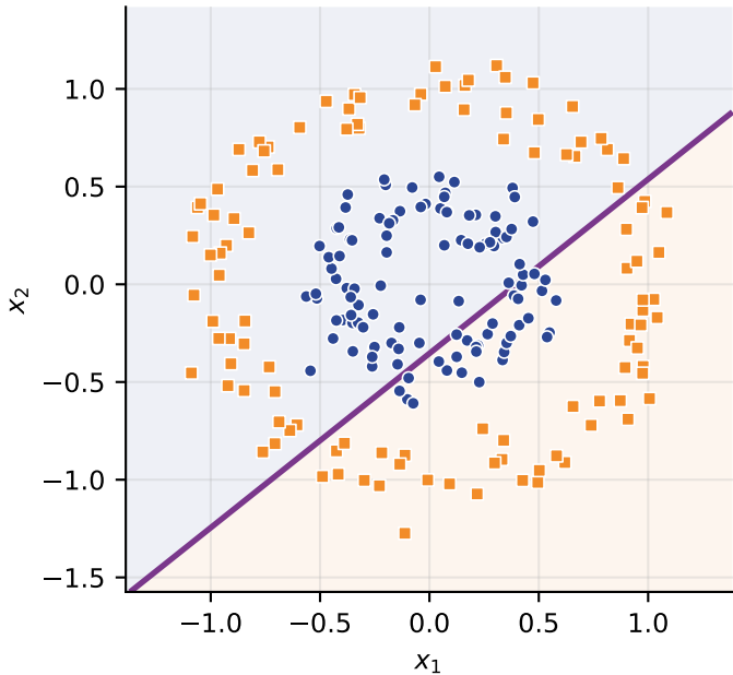
Raw 2-D: a line scores 0.5682
