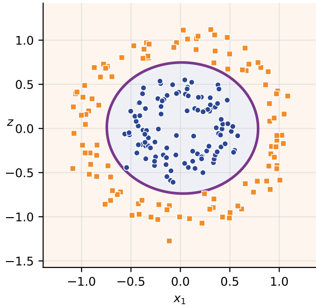
Back in 2-D: the plane is a circle poly kernel scores 1.0000
