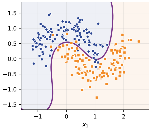
RBF, \gamma = 1 64 SVs, 5-fold CV 0.9458
