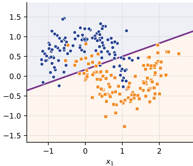
linear 86 SVs, 5-fold CV 0.8583
