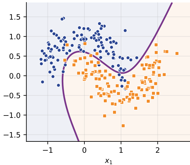
poly, degree 3 53 SVs, 5-fold CV 0.9417
