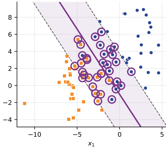
C = 0.01 : 35 SVs, width 5.214 train accuracy 0.9625
