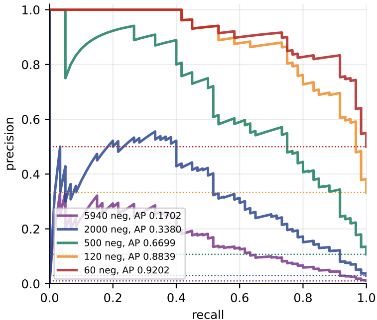
Five PR curves, same scores -- they do not
