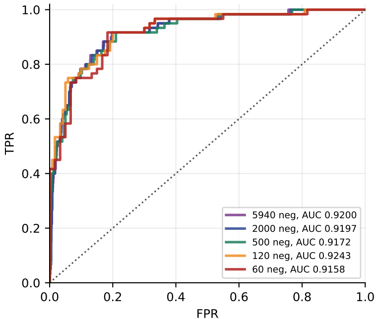
Five ROC curves, same 60 positives -- they coincide
