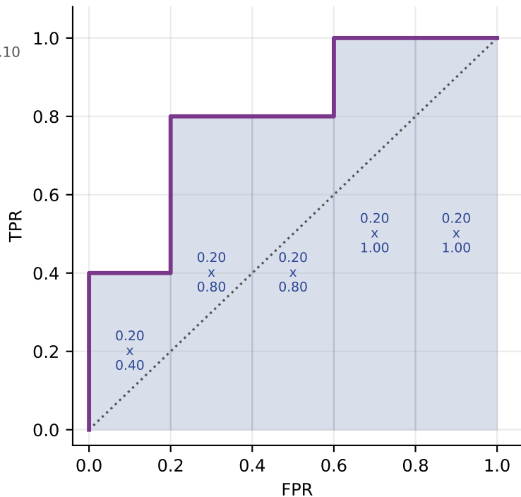
Five strips, area 0.80 = roc_auc_score 0.80
