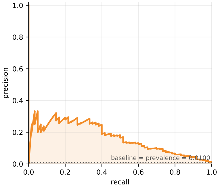
PR: average precision 0.1702 -- the same model
