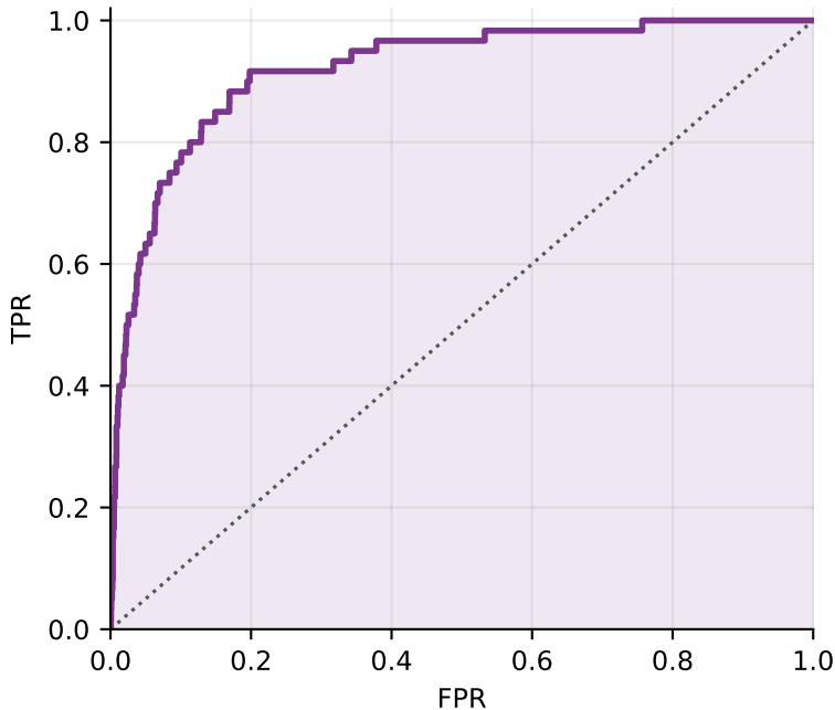
ROC: AUC 0.9200 -- this looks like a good model
