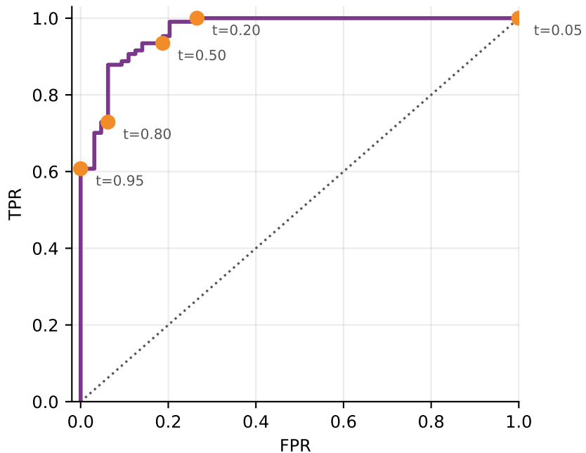
One curve, AUC 0.9661, and the thresholds live on it
