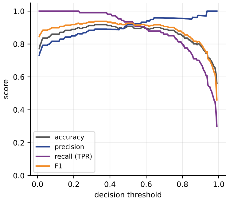
Four metrics that all depend on the threshold
