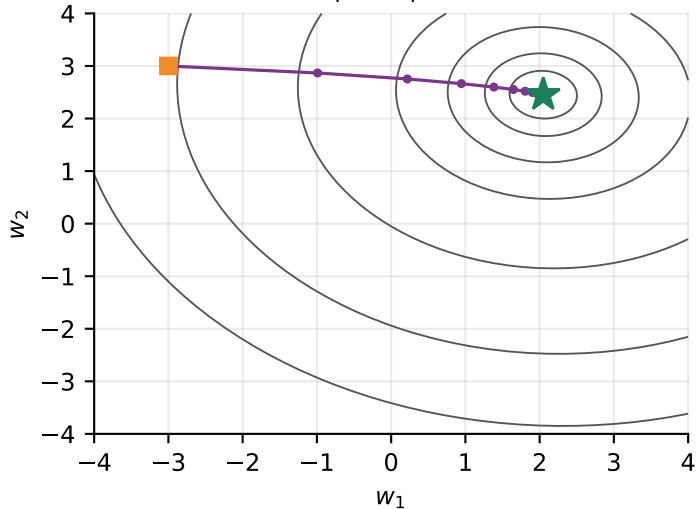
standardised: sd 1.0 and sd 1.0 60 steps, step size 0.2
