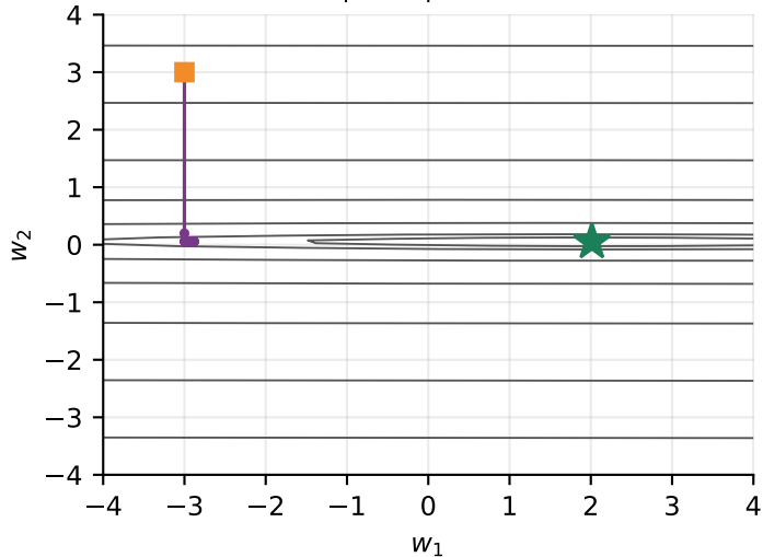
raw: sd 1.0 and sd 50 60 steps, step size 0.0002
