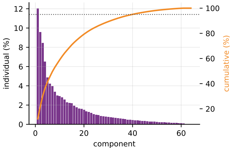
digits, 64 pixels: the scree plot and its running total
