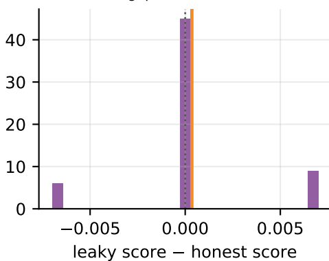
B impute on all data (accuracy, 30% missing) mean gap +0.0003, t = +0.8
