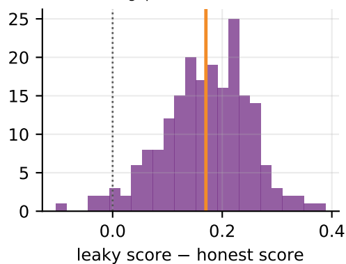
C drop hard rows on all data ( R^2 , worst 10%) mean gap +0.1702, t = +29.9
