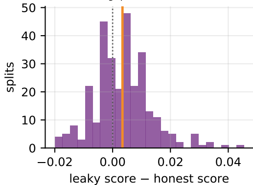
A scale on all data (accuracy, n_{train} = 20 ) mean gap +0.0034, t = +6.0
