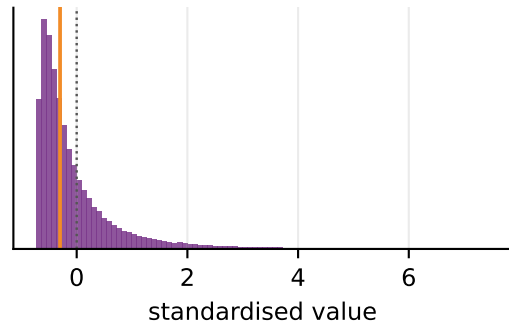
lognormal g_1 = +6.03 , excess g_2 = +86.43
