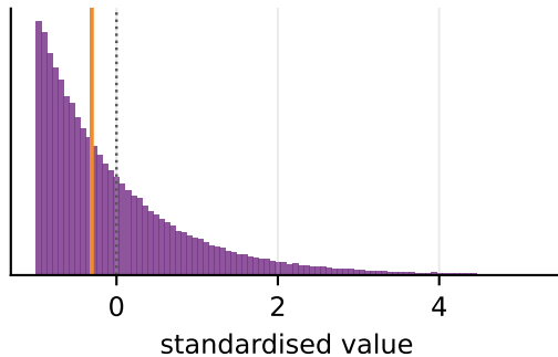
exponential g_1 = +2.00 , excess g_2 = +6.06
