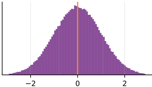
normal g_1 = -0.00 , excess g_2 = +0.01
