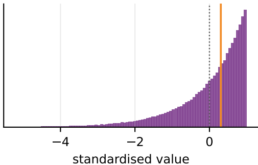
left-skewed g_1 = -2.00 , excess g_2 = +5.98
