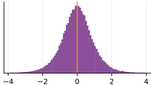
Student t_5 g_1 = -0.01 , excess g_2 = +4.62
