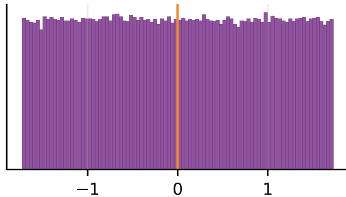
uniform g_1 = +0.00 , excess g_2 = -1.20
