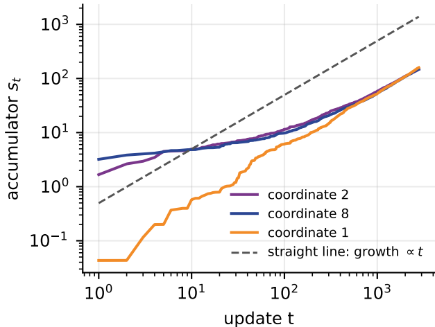
The sum only ever grows
