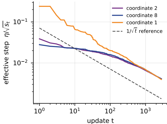
So the effective learning rate decays
