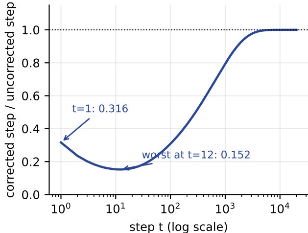
Uncorrected, the early steps are far too big
