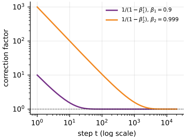
Both decay to 1, at very different speeds
