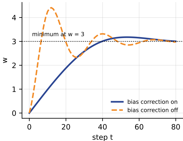
Adam on f(w) = (w - 3)^2 , \eta = 0.1
