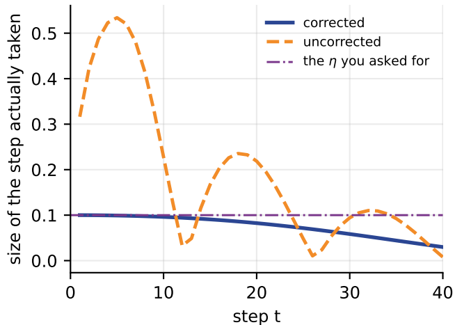
Uncorrected, the early steps run away
