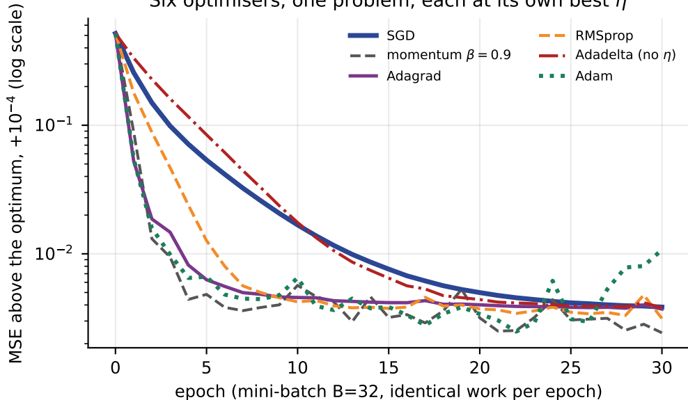
Six optimisers, one problem, each at its own best \eta
