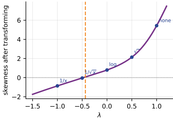
one family, indexed by \lambda
