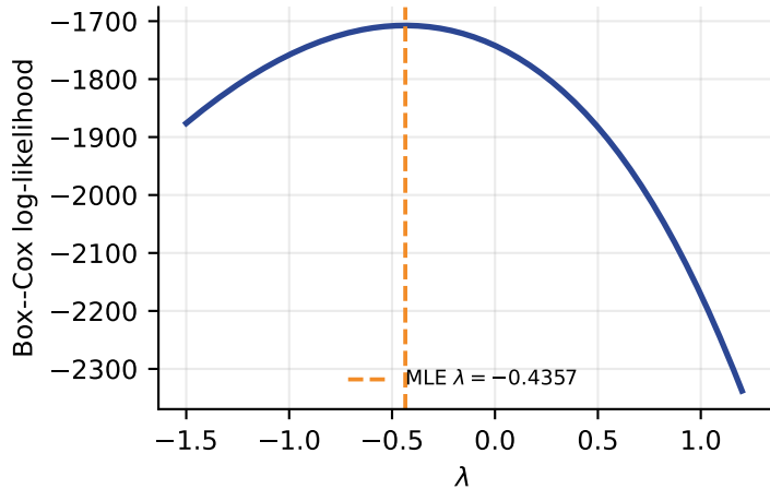
scipy maximises this, not the skewness
