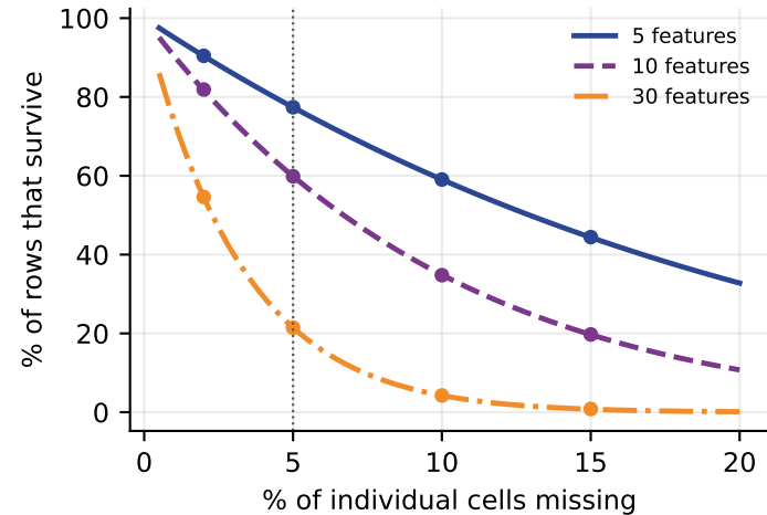
listwise deletion: (1 - p)^d
