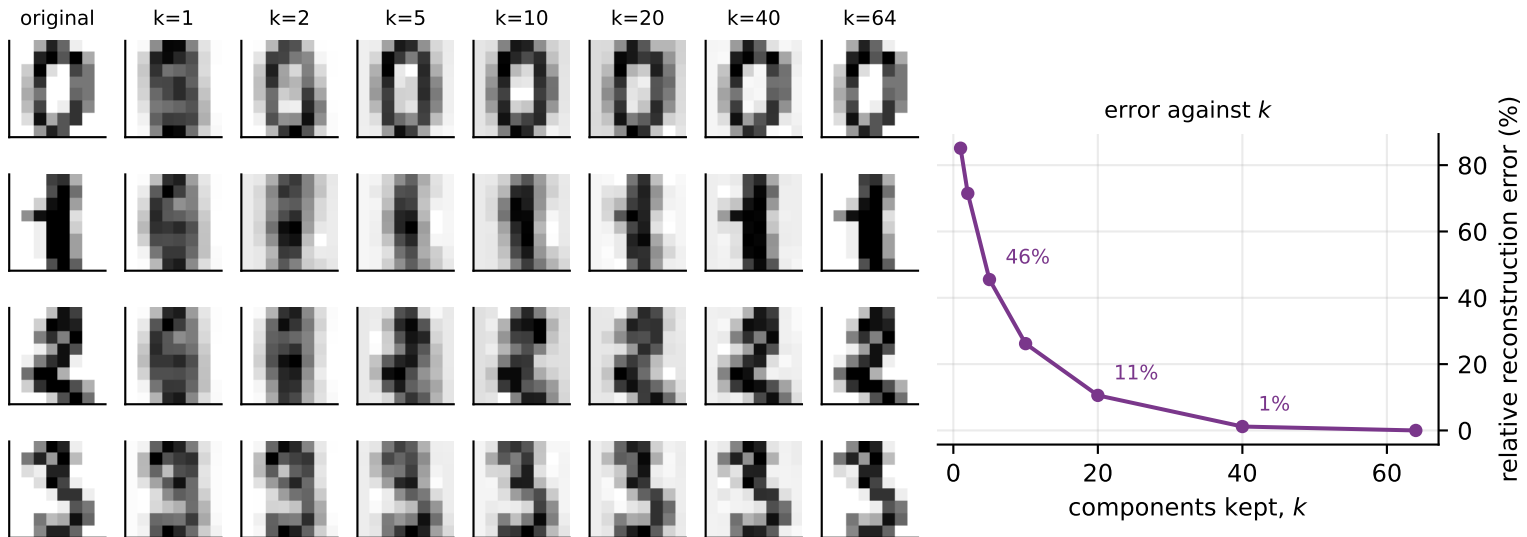
digits: 64 pixels reconstructed from k principal components
