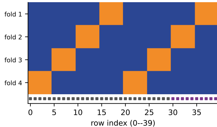
GroupKFold(4)
