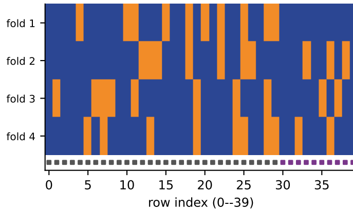
ShuffleSplit(4, test=25%)
