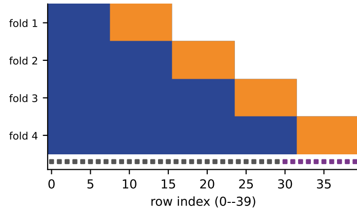
TimeSeriesSplit(4)
