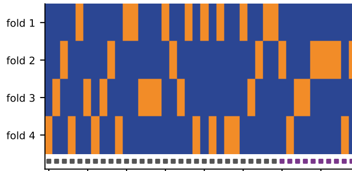
ShuffleSplit(4, test=25%)
