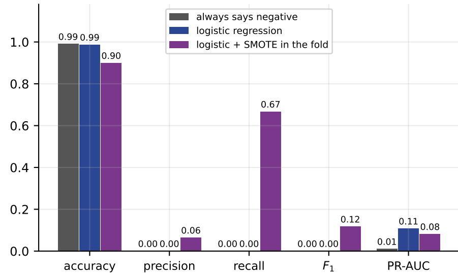
1% positives: accuracy cannot tell these three apart
