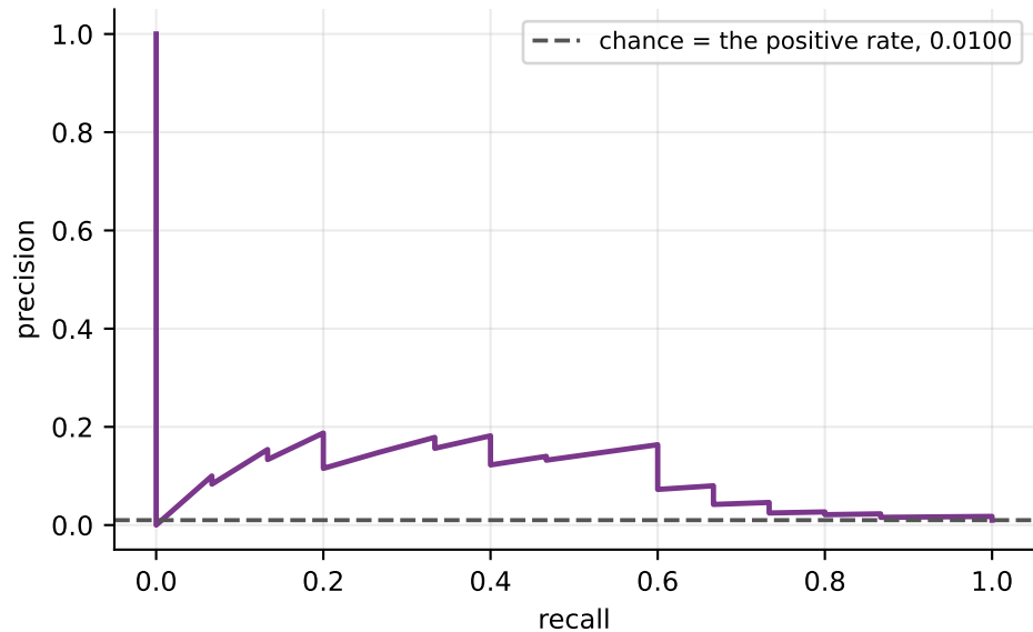
precision--recall curve, PR-AUC 0.1075
