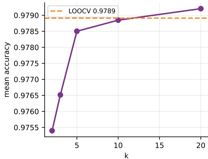
bias: small k trains on less data
