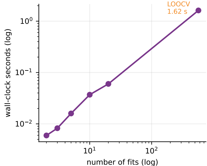
cost: linear in k
