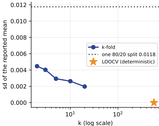
variance of the estimate
