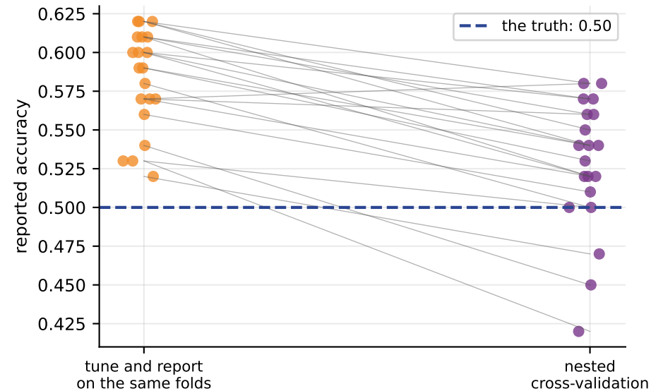
100 rows, 200 pure-noise features, coin-flip labels
