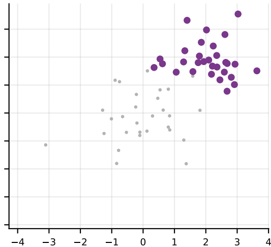
random undersample 60 rows, 30 positive
