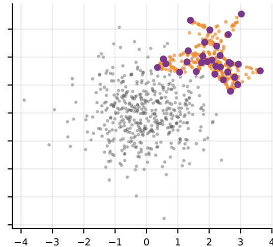
SMOTE 940 rows, 470 positive
