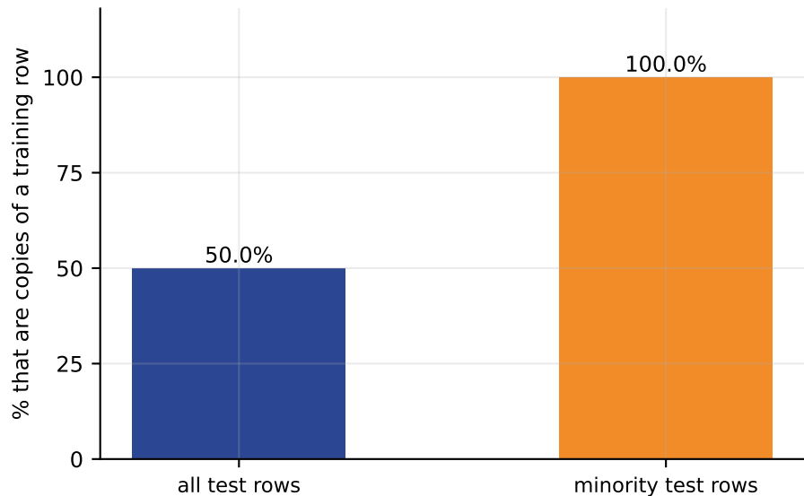
why: oversampling puts the same row on both sides
