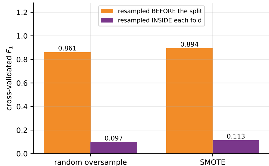
the same code, one line moved
