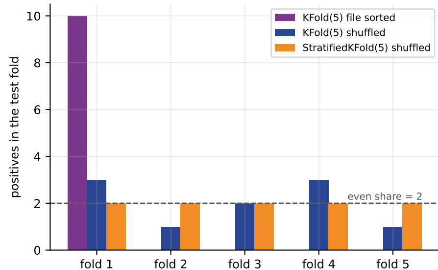
200 rows, 10 positives (5%)
