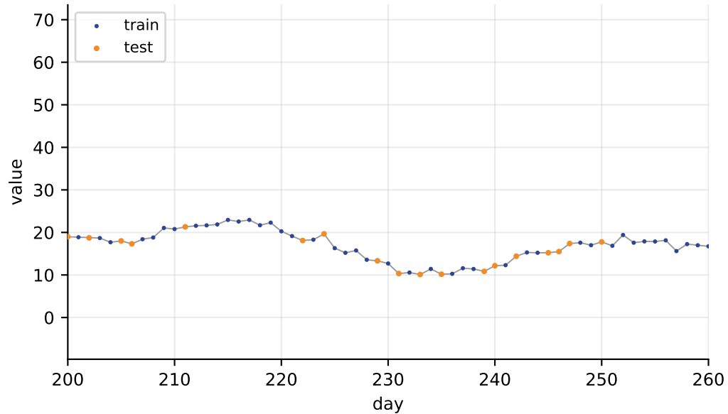
random split, zoomed to 60 days: R^2 = +0.9975
