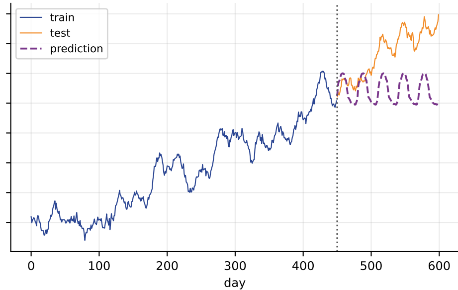
time-ordered split: R^2 = -2.7683
