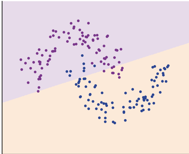
logistic regression on x_1, x_2 test 0.9056
