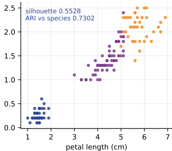
k-means, k = 3
