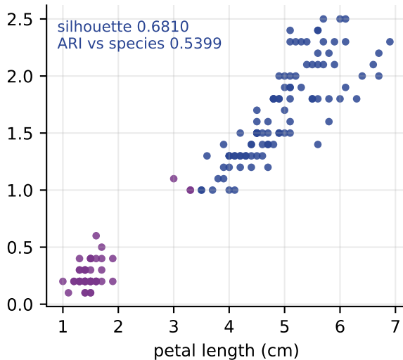
k-means, k = 2
