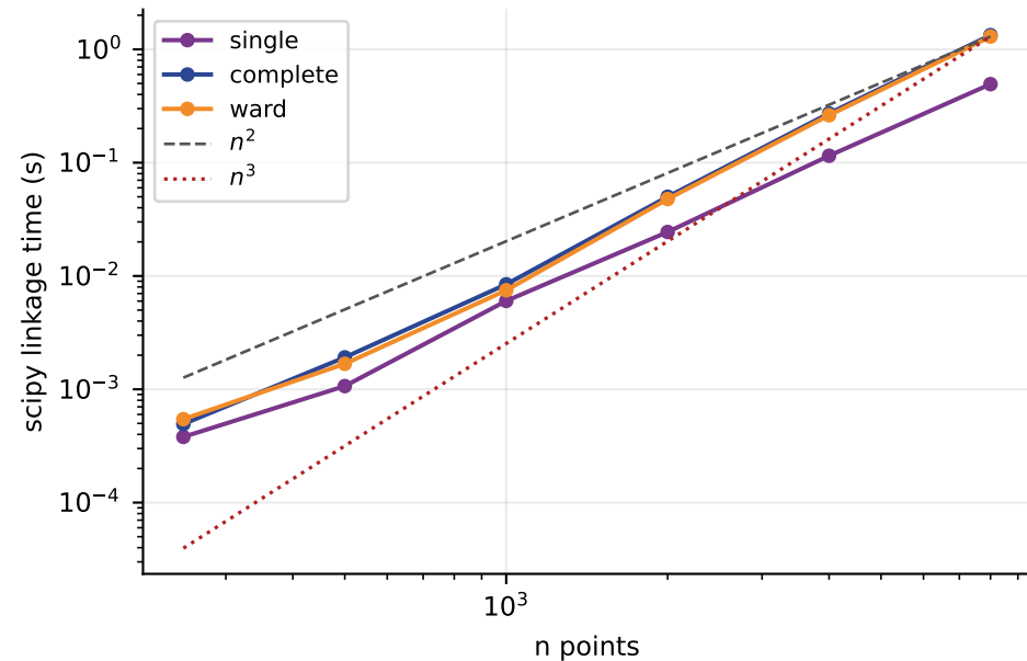
measured: close to n^2 , not n^3
