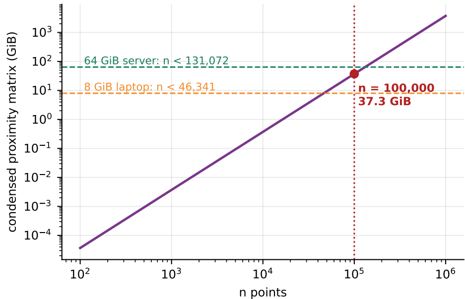
space: n(n-1)/2 float64 entries
