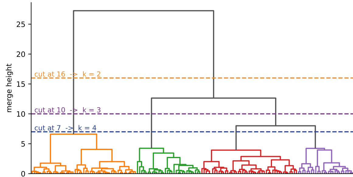
iris, standardised, Ward linkage
