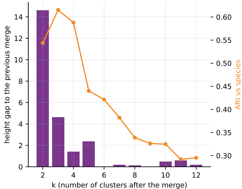
the gap heuristic: biggest jump at k = 2
