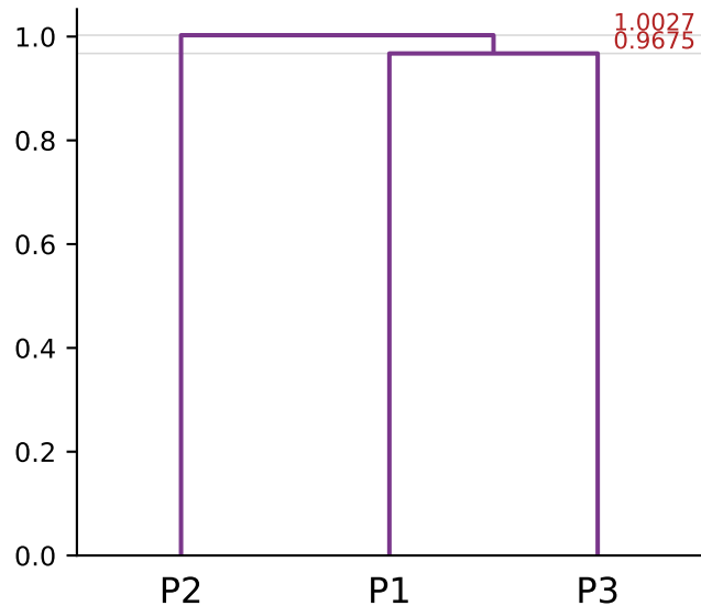
ward: heights 0.9675 then 1.0027
