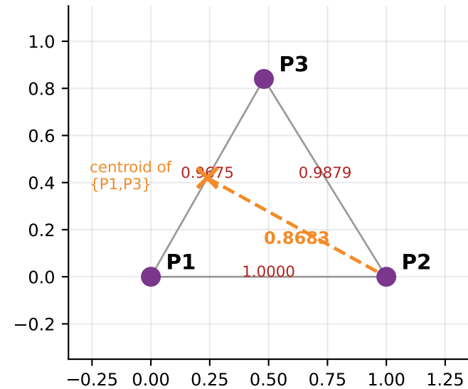
merge P1,P3 at 0.9675; the new centroid is 0.8683 from P2
