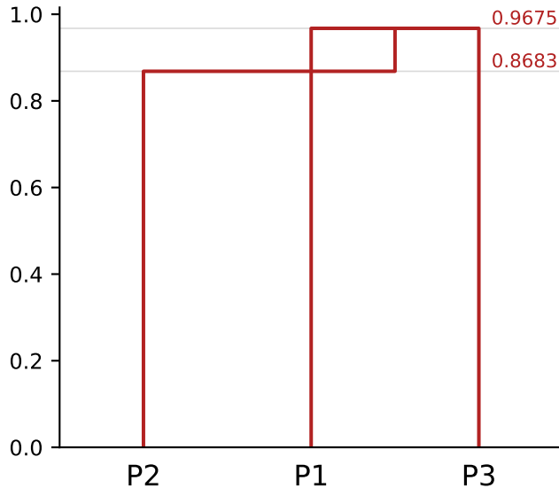
centroid: heights 0.9675 then 0.8683
