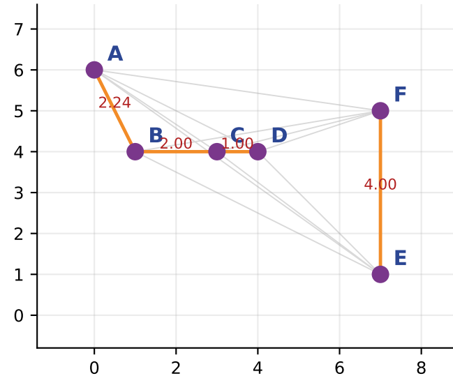
six points, all 15 distances (four shortest marked)
