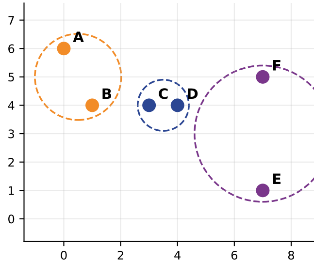
complete linkage, cut at k = 3
