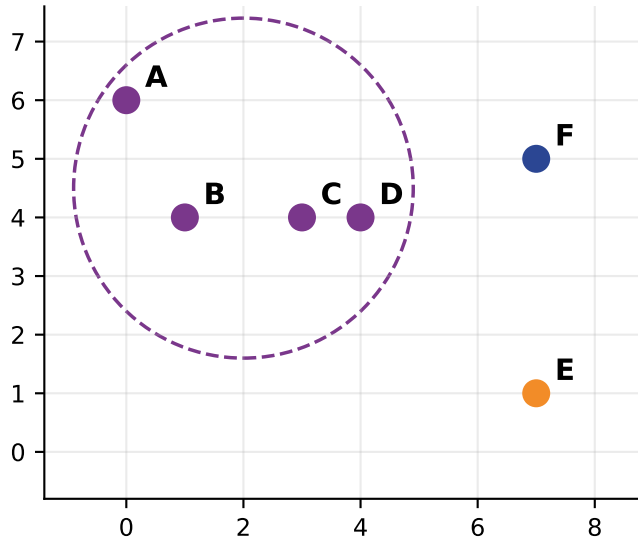
single linkage, cut at k = 3
