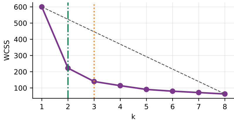
iris, standardised: WCSS. chord rule k = 3 , drop-ratio rule k = 2
