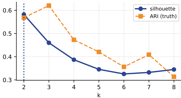
iris, standardised: silhouette peaks at k = 2
