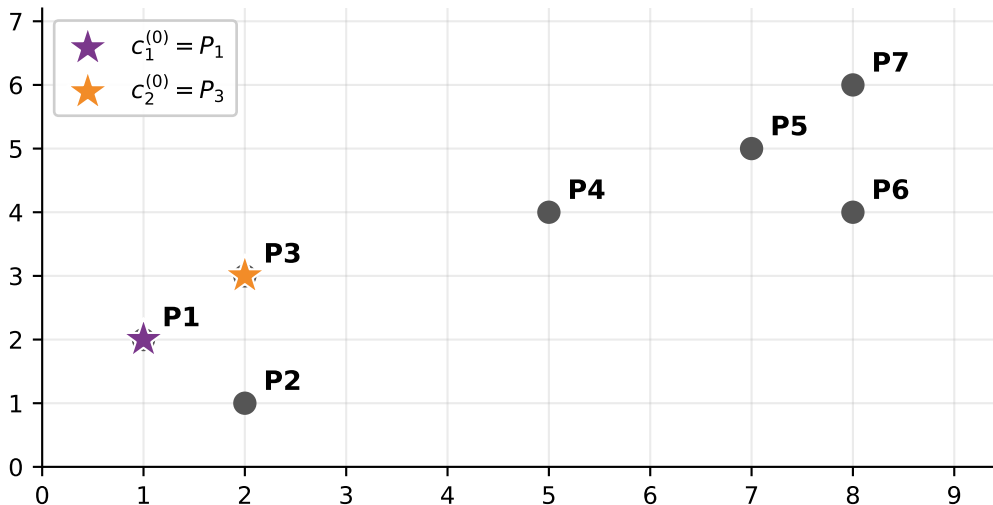
Seven points, k = 2 , and two deliberately bad initial centroids
