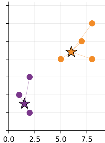
3. assignment WCSS = 16.7400
