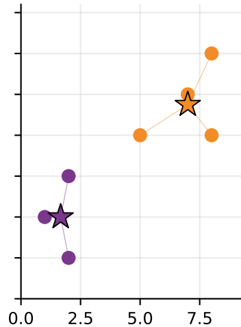
5. assignment WCSS = 11.4167
