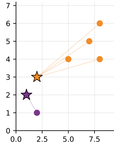
1. assignment WCSS = 123.0000
