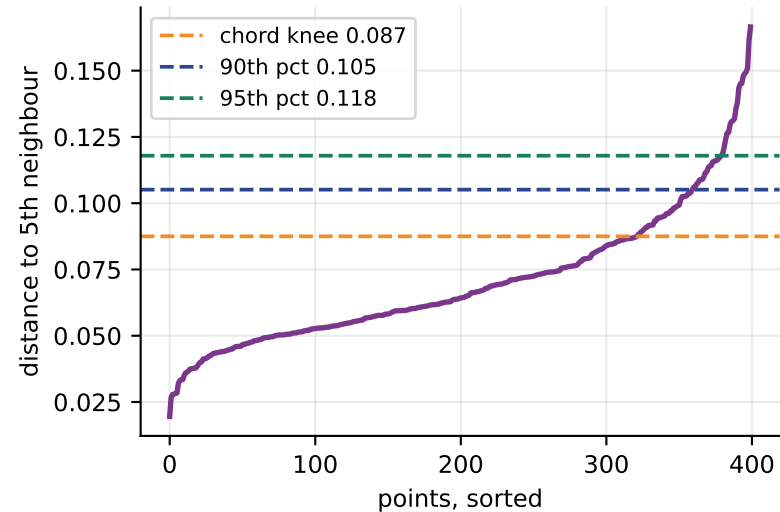
k-distance graph, minPts = 5
