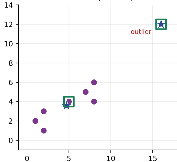
outlier at (16, 12.0)
