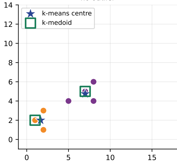
no outlier
