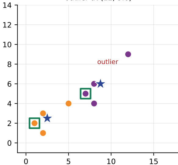
outlier at (12, 9.0)
