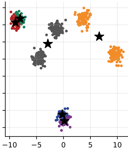
random seed 7 WCSS 5010.6, ARI 0.583
