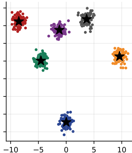
k-means++, one start WCSS 431.5, ARI 1.000
