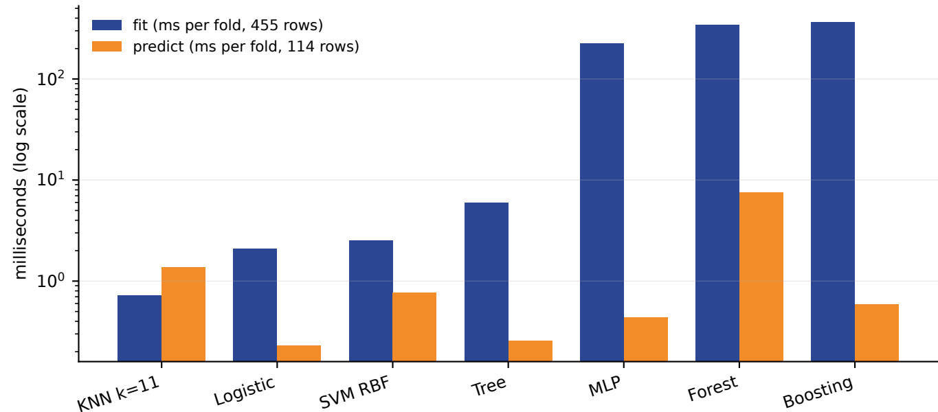
Same data, same score to within a fold's noise, a factor of 507 in cost
