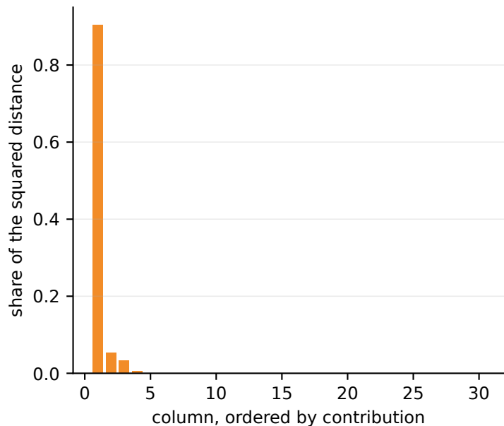
One column supplies 0.9045 of the distance between two unscaled patients
