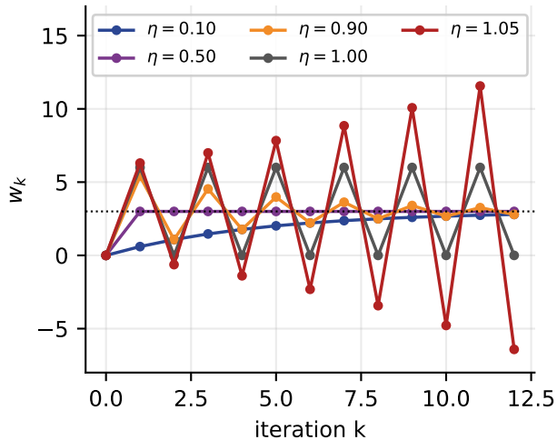
Trajectory on f(w) = (w - 3)^2 , w_0 = 0
