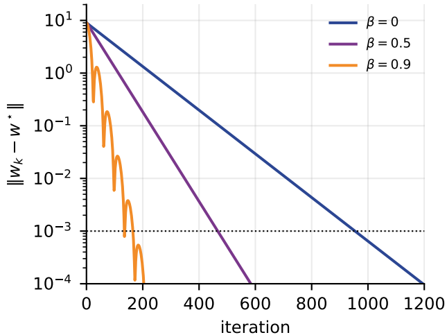
Distance to the optimum
