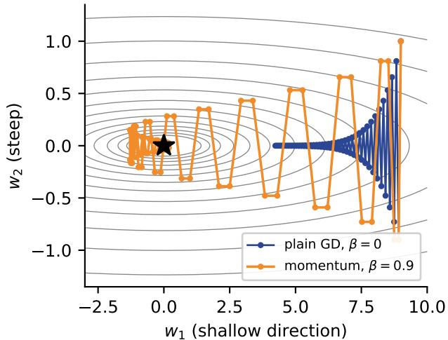
80 steps in a ravine, same \eta = 0.475
